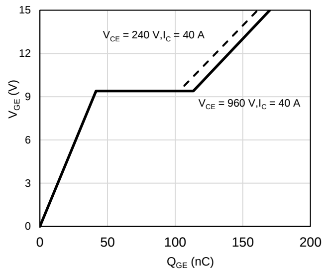
Figure 16: Gate-Charge Characteristics
