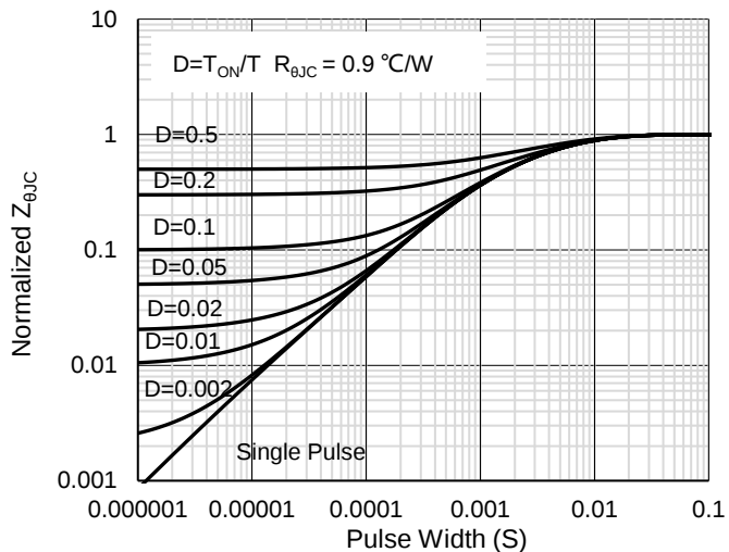
Figure 21: Normalized Maximum Diode Transient Thermal Impedance
