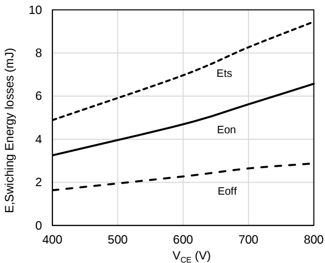
Figure 15: Switching Energy losses vs. Collector Emitter Voltage
